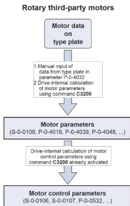
Fig. 306: Procedure and results of "C3200 Command Calculate motor data"
