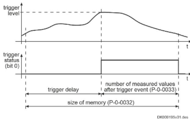
Fig. 354: Trigger delay: Number of measured values after trigger event
