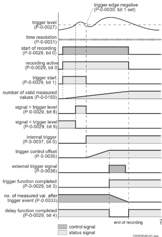
Fig. 353: External trigger with offset measurement (P-0-0028 (/redirect/patternMatch?code=P-0-0028&redirectOrigin=ID1765338_227647791); bit 1 = 1)
