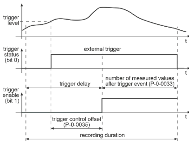
Fig. 356: Trigger control offset
