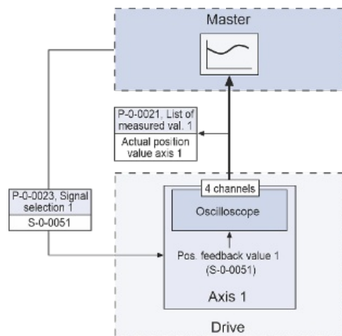
Fig. 351: Example of signal selection
