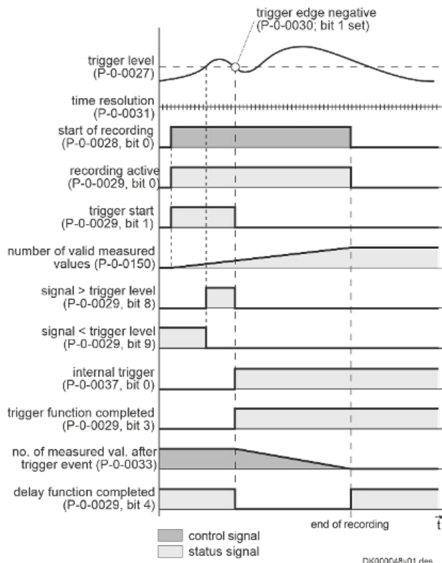
Fig. 352: Internal trigger without offset measurement (P-0-0028 (/redirect/patternMatch?code=P-0-0028&redirectOrigin=ID1765338_227647791); bit 1 = 0)
