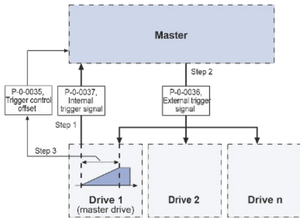
Fig. 355: Application for trigger source "External" with determination of trigger offset
