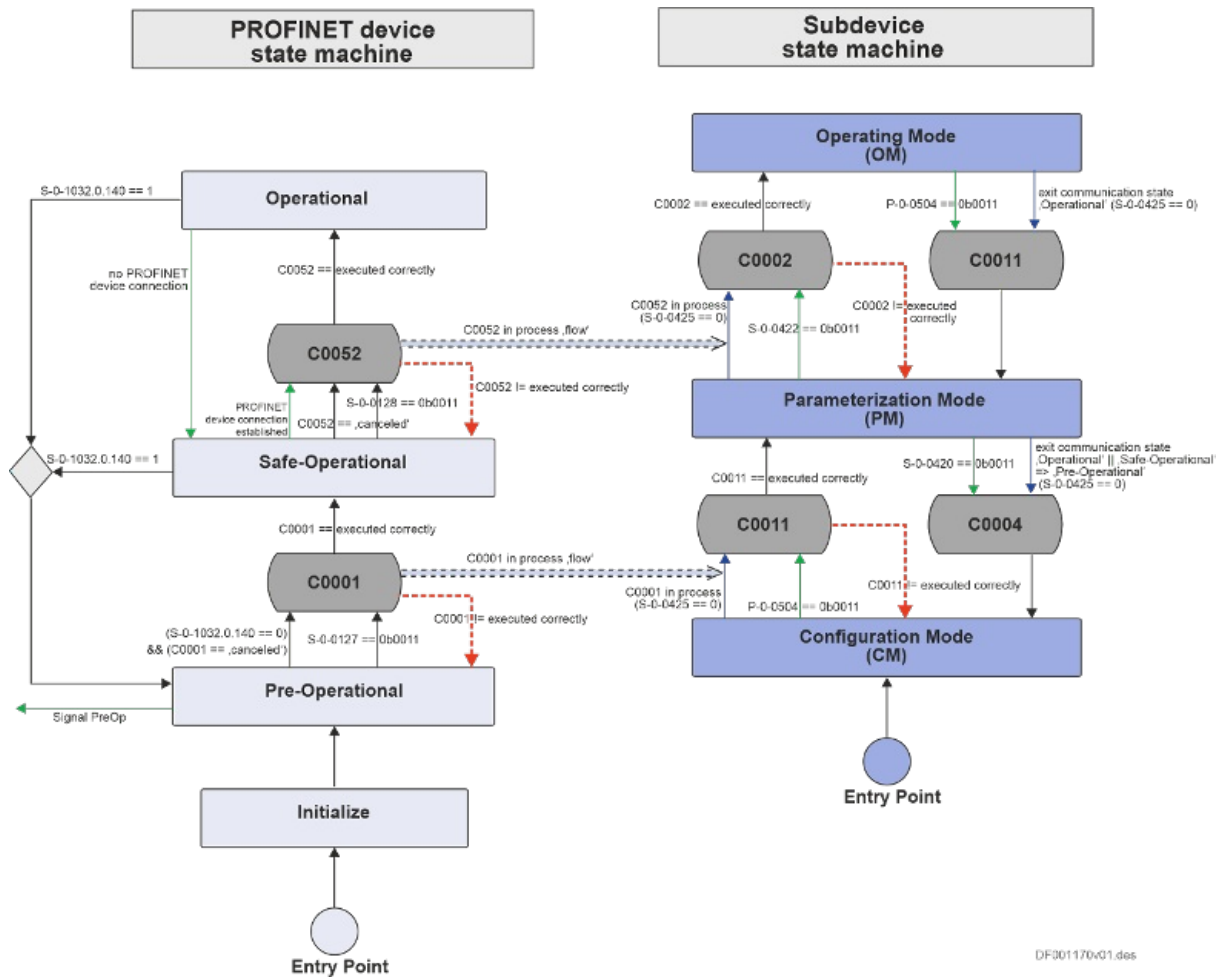
Fig. 88: PROFINET® IO device state machine
